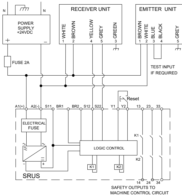
Figure 4 – SRUS Connection Details
