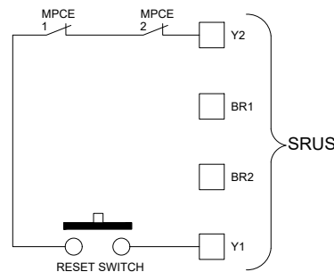
Figure 2- Cross-monitoring of MPCEs – Manual Reset
