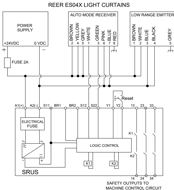
Figure 5 – SRUS Connection Details for REER ES04X
