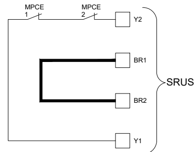
Figure 3- Cross-monitoring of MPCEs –Auto Reset
