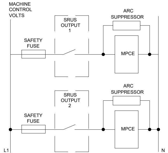
Figure 7 - Safety Output Connection (Two MPCEs)
