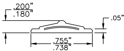
SECTION: 'A'-'A' Scale 2:1
