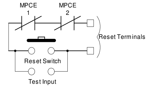
Figure 10 Connection of Test Input
