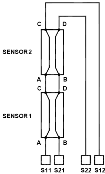
Figure 4 – Sensors in Series
