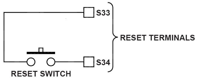
Figure 6 – Manual Reset
